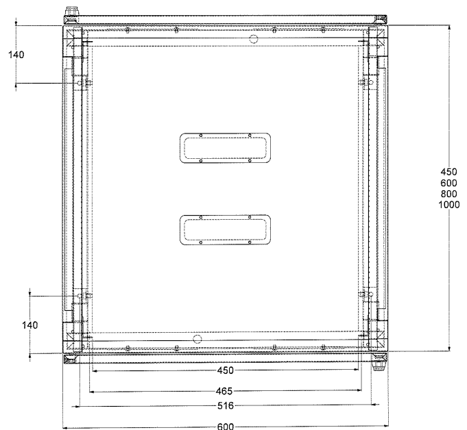
600 WIDE PLAN
