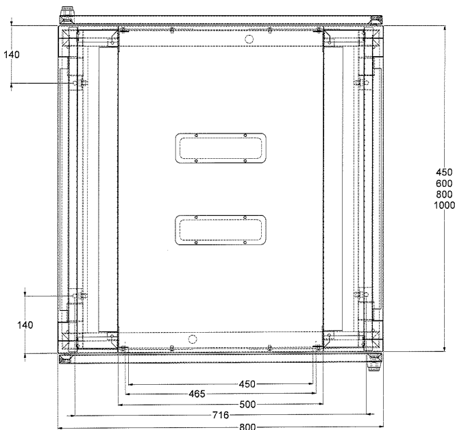
800 WIDE PLAN
